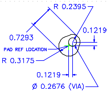
0.75 mm PITCH. LOAD BOARD PAD
