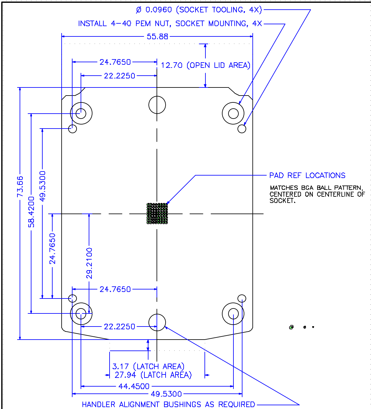
0.75 mm PITCH. LOAD BOARD PAD
